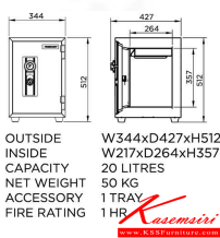
SS2 Outside Dimension (WxDxH)[MM.] 344 X 427 X 512 Inside Dimension (WxDxH)[MM.] 217 X 264 X 357 Net Weight 50 KG Capacity 20 Litres
