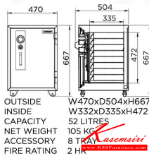
SMT Outside Dimension (WxDxH)[MM.] 470 X 504 X 667 Inside Dimension (WxDxH)[MM.] 332 X 335 X 472 Net Weight 105 KG Capacity 52 Litres
