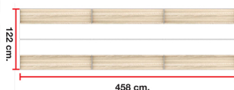
NM-611 (SIZE : 458 x 122 x 160 cm.) WORKSTATION SERIES
