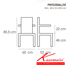
PN92258AL/AT Dim. 60 x 53 x 85.5 cm color : blue-antique
