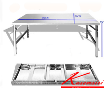
JK-205 W150xD70xH75 CM.
