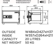
SS1D4 Outside Dimension (WxDxH)[MM.] 484 X 427 X 372 Inside Dimension (WxDxH)[MM.] 357 X 264 X 217 Net Weight 50 KG Capacity 20 Litres
