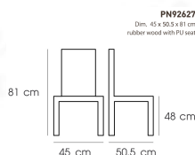
PN92627 Dim. 45 x 50.5 x 81 cm rubber wood with PU seat
