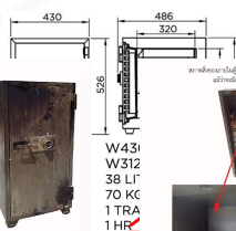
SS70D4OV Outside Dimension [WxDxH][MM.] 430 X 486 X 526 Inside Dimension [WxDxH][MM.] 312 X 320 X 380 Net Weight 70 KG Capacity 38 Litres
